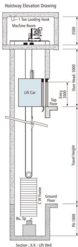
Section : X-X - Lift Well
