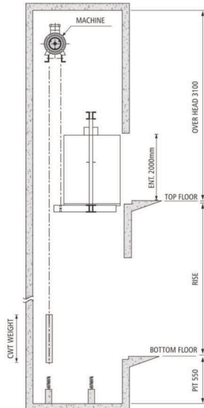
HOISTWAY ELEVATION PLAN
