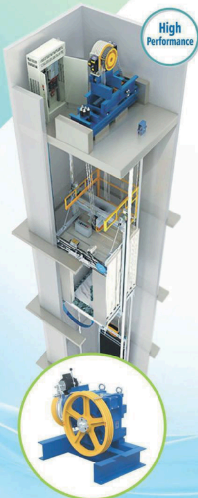
Geared Traction Machine
